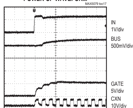
POWER-UP WAVEFORM
