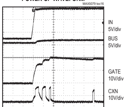
POWER-UP WAVEFORM
