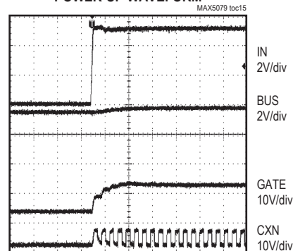
POWER-UP WAVEFORM
